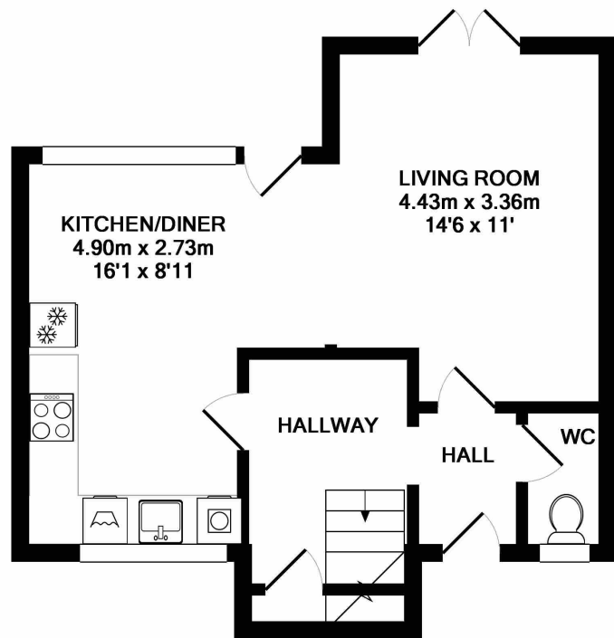
GROUND FLOOR APPROX. FLOOR AREA 41.9 SQ.M. (451 SQ.FT.)
