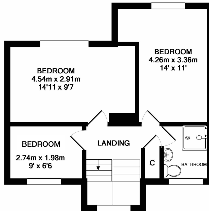
1ST FLOOR APPROX. FLOOR AREA 41.5 SQ.M. (447 SQ.FT.)
